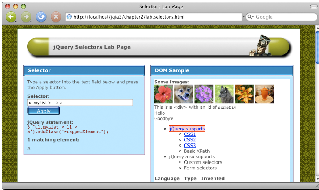
Figure 2.4 With the selector ul.myList > li > a , only the direct children of parent nodes are matched
