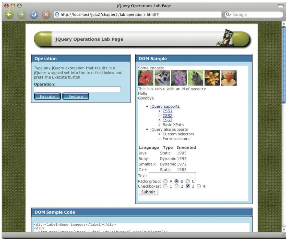
Figure 2.6 The jQuery Operations Lab helps us see how wrapped sets can be created and managed.
