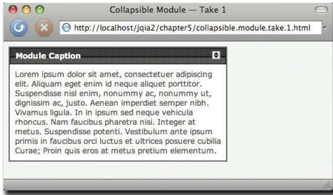
Figure 5.2a We'll create our own dashboard modules which consist of two parts: a banner with a caption and 'roll up' button, and a body in which data can be displayed
