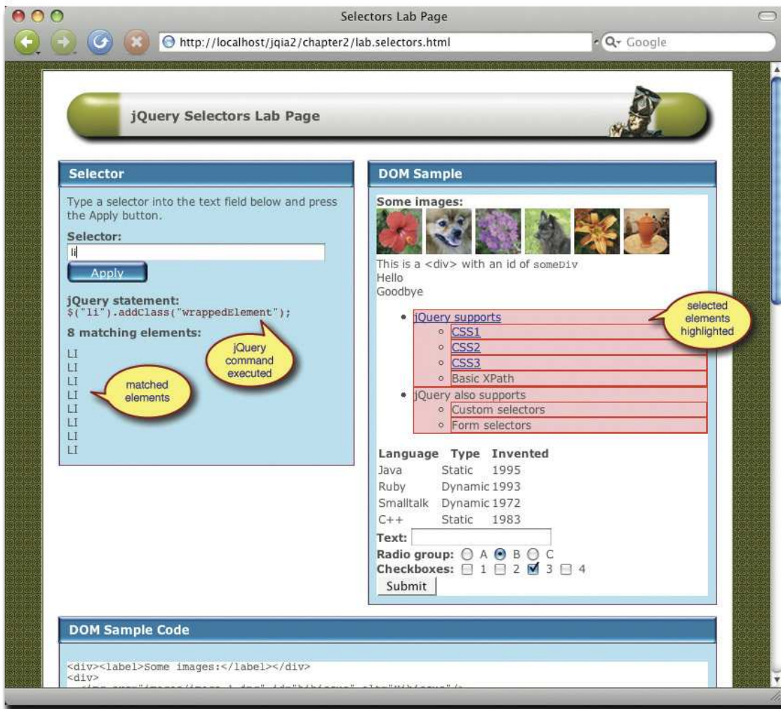
Figure 2.2 A selector value of li matches all <li> elements when applied as shown by the displayed results
