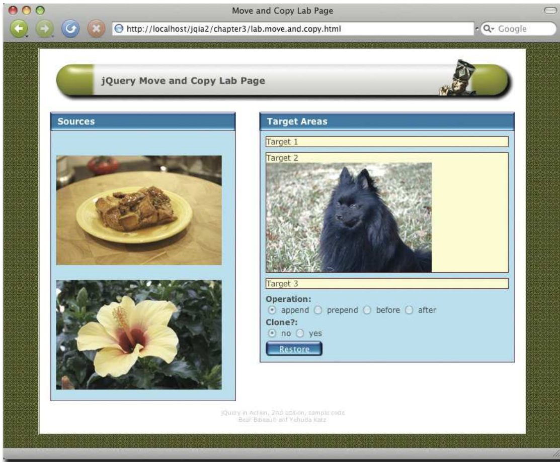
Figure 3.5 Cozmo has been added to the end of Target 2 as a result of the append operation
