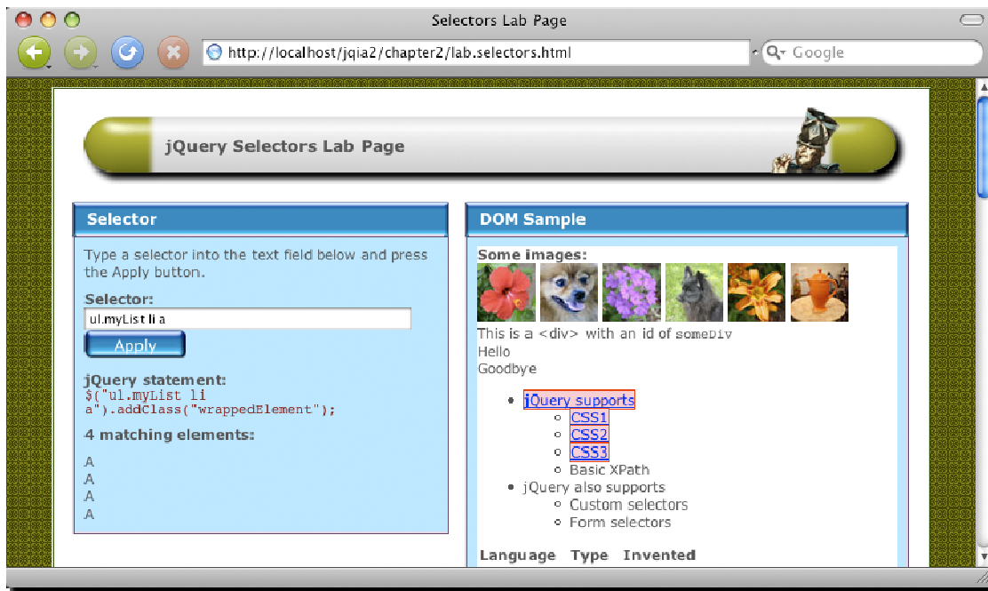
Figure 2.3 All anchor tags that are descendants, at any depth, of an <li> element are selected by ul.myList li a
