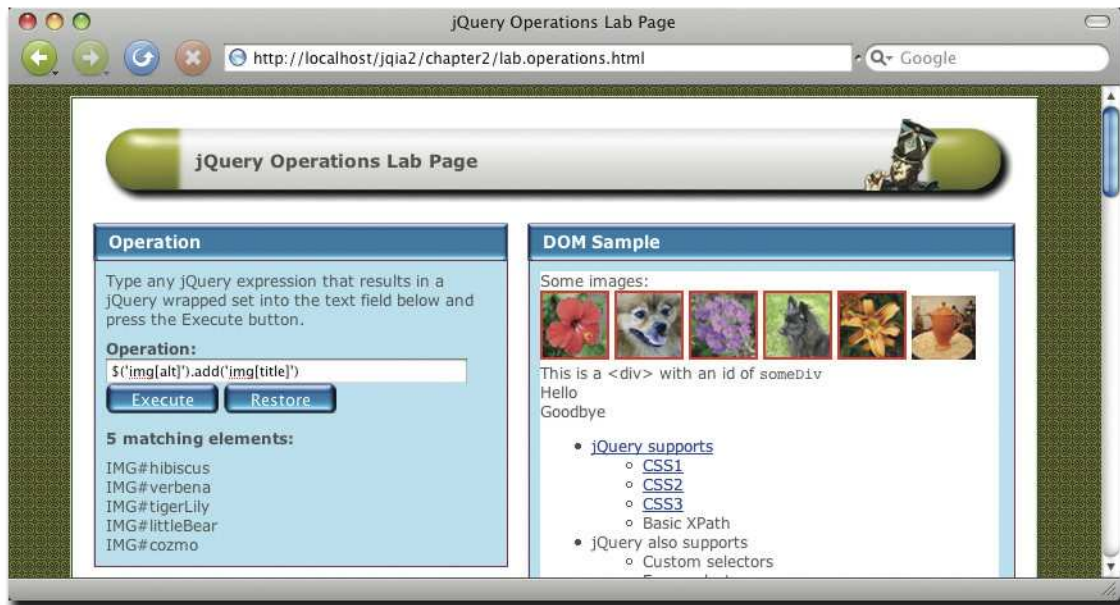
Figure 2.7 The expected image elements, those with an alt or title attribute, have been matched by the jQuery expression
