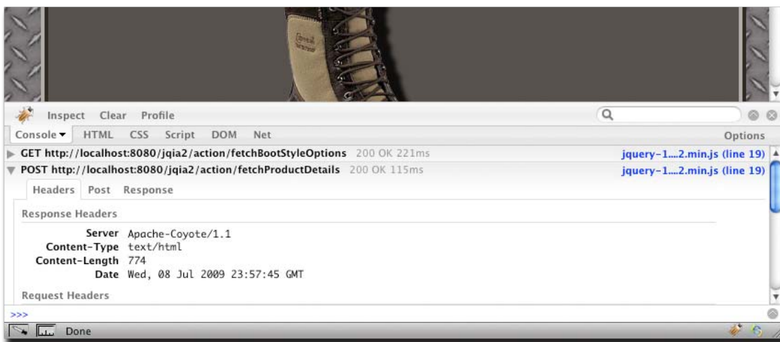
Figure 8.4 An inspection of the Firebug console shows that we're making a POST request when we should be making a GET
